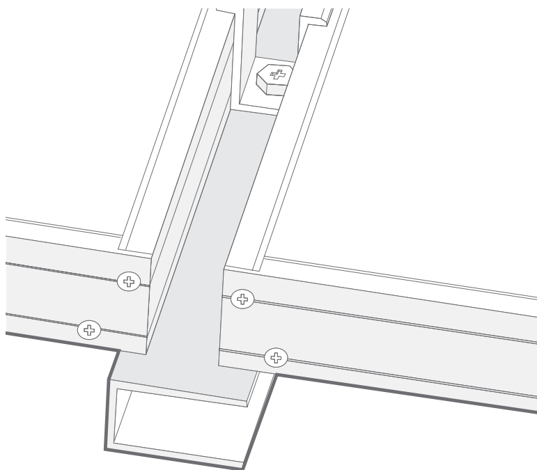
CLIP MOUNTING
